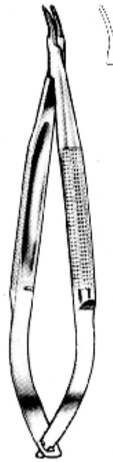
BARRAQUER 22.0282.13 13.0cm
