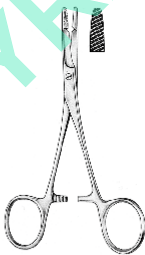
OLSEN-HEGAR 22.0172.17 17.0cm
