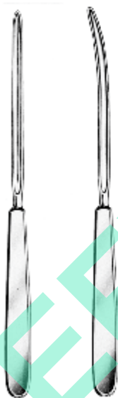
PAYR 22.0cm 22.0420.22 22.0422.22
