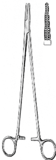
JAMISON 22.0150.23 23.5cm
