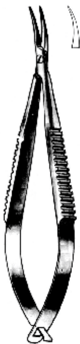
CASTROVIEJO 22.0261.09 9.0cm
