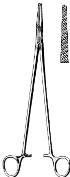
WANGENSTEEN 22.0146.27 27.0cm
