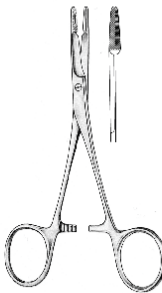
OLSEN-HEGAR 22.0174.17 17.0cm
