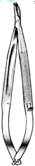
BARRAQUER 22.0280.11 11.0cm
