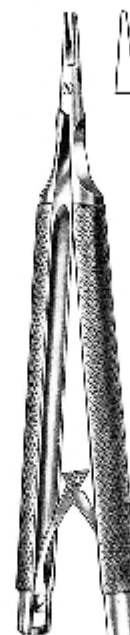
CASTROVIEJO 22.0344.12 12.0cm
