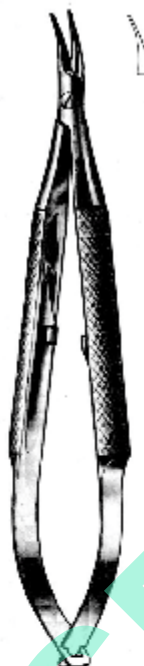
BARRAQUER-TROUTMAN 22.0271.10 10.0cm
