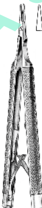
CASTROVIEJO 22.0342.13 13.0cm
