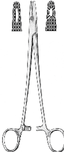
METZENBAUM
