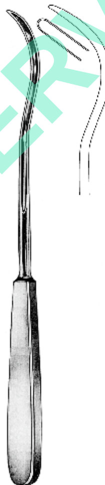
KIRSCHNER 22.0434.25 25.0cm
